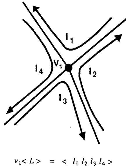
Figure 10 - 11. V \langle L \rangle adjacency relationship example
