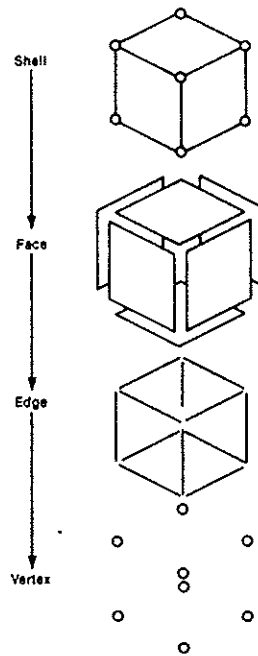
Figure 4 - 4. Top-down hierarchical representation of topological elements
