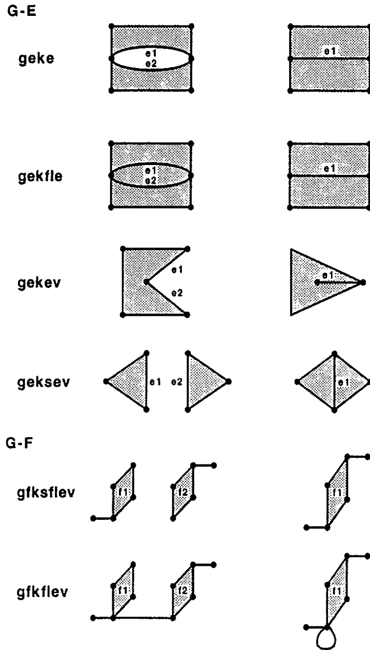
Figure 19 – 3. Action of the non-manifold topology operators
